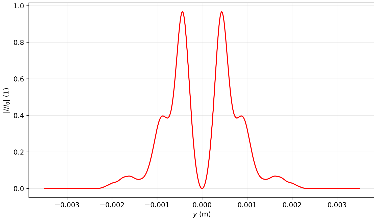
Intensity profile I(x=0, y, z=1.911)/I_0 , \text{Pin}=6.0\text{Pcr} , artificial time
